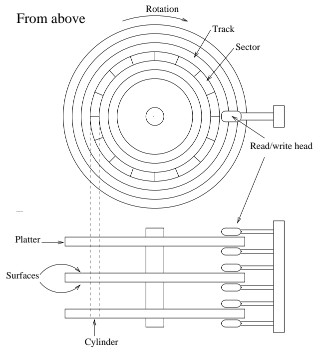
Figure 4.1: A schematic picture of a hard disk.
